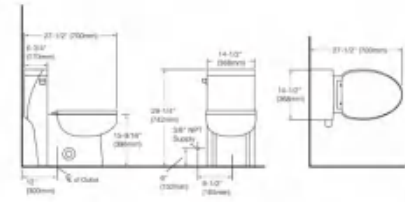
Flushing system: Siphonic S trap: 300mm
