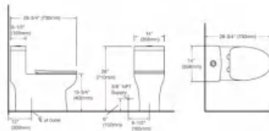
Flushing system: Siphonic S trap: 300mm
