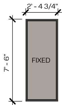
TYPE PA2 1 PANEL FIXED WINDOW
