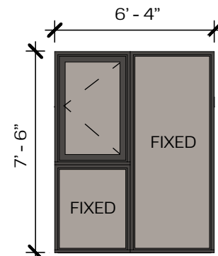
TYPE PE1 CASEMENT OVER FIXED + FIXED WINDOW
