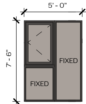
TYPE PE2 CASEMENT OVER FIXED + FIXED WINDOW
