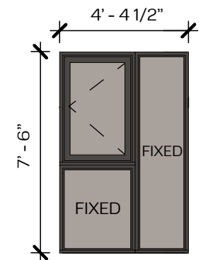
TYPE PE3 CASEMENT OVER FIXED + FIXED WINDOW
