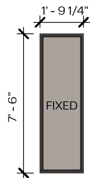
TYPE PA3 1 PANEL FIXED WINDOW
