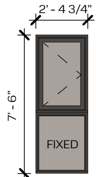
TYPE PF1 CASEMENT OVER FIXED
