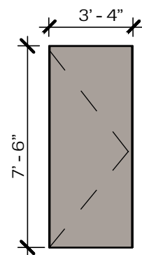
TYPE PJ2 EXTERIOR MASONITE SWING DOOR *PICK COLOR FROM SIDING COLOR PALETTE*
