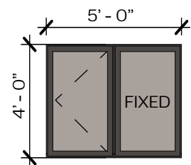
TYPE D1 CASEMENT + FIXED WINDOW OPERATION VARIES
