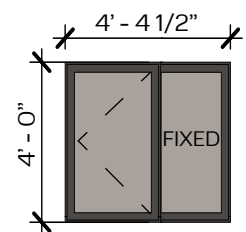
TYPE D2 CASEMENT + FIXED WINDOW OPERATION VARIES
