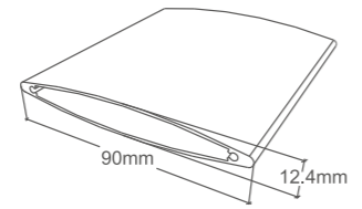
▲ Fixed Shutter
