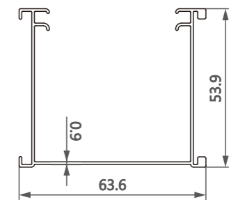
型号/Item No.-13031331 米重/Weight-0.544kg/m
