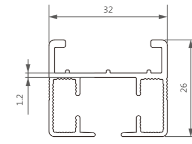
型号/Item No.-1514575 米重/Weight-0.444kg/m
