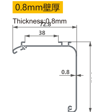
型号/Item No.-11182494 米重/Weight-0.449kg/m
