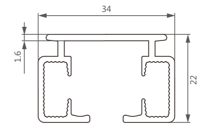
型号/Item No.-13031150 米重/Weight-0.473 kg/m
