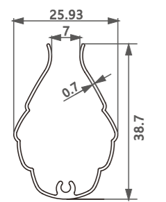
型号/Item No.-11181162 米重/Weight-0.212kg/m
