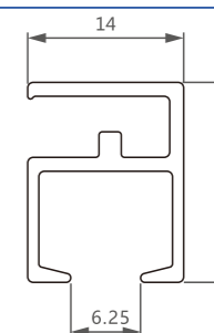
型号/Item No.-1514858 米重/Weight-0.198kg/m
