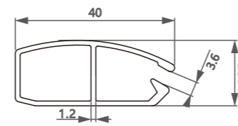
型号/Item No.-110172 米重/Weight-0.382kg/m
