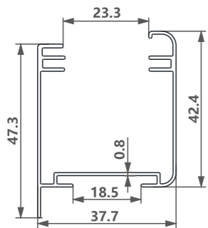
型号/Item No.-1202680-0.8 米重/Weight-0.409kg/m
