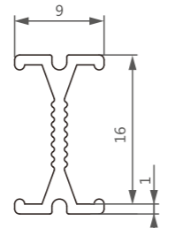
型号/Item No.-1404128 米重/Weight-0.109kg/m
