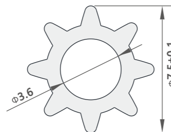
型号/Item No.-1303356 米重/Weight-0.053kg/m
