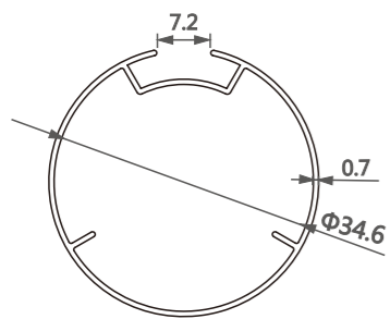
型号/Item No.-1110110 米重/Weight-0.246kg/m
