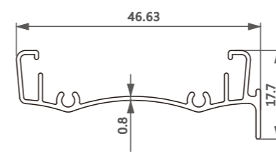
型号/Item No.-111344 米重/Weight-0.251kg/m
