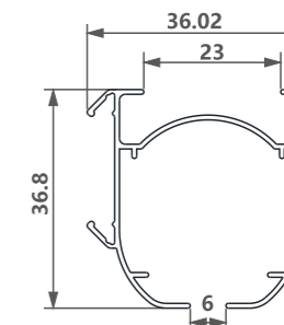
型号/Item No.-111367 米重/Weight-0.327kg/m
