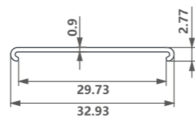
型号/Item No.-1202720 米重/Weight-0.089kg/m
