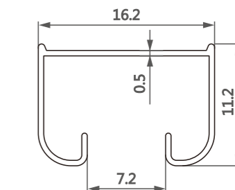
型号/Item No.-1303758 米重/Weight-0.065kg/m
