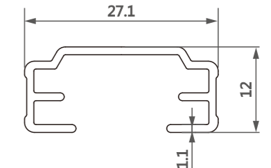
型号/Item No.-1514239 米重/Weight-0.197kg/m
