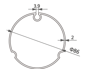
型号/Item No.-1116945 米重/Weight-1.658kg/m
