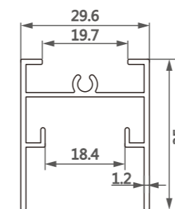
型号/Item No.-1303755 米重/Weight-0.399kg/m
