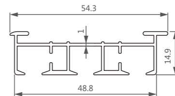
型号/Item No.-1514956 米重/Weight-0.415kg/m
