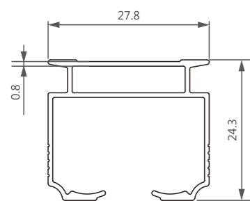
型号/Item No.-1514770 米重/Weight-0.271kg/m
