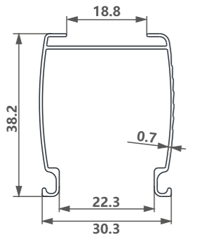
型号/Item No.-1116961-0.7 米重/Weight-0.244kg/m
