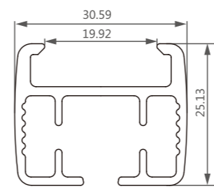
型号/Item No.-1303633 米重/Weight-0.530kg/m
