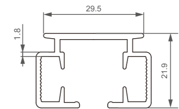
型号/Item No.-13031001 米重/Weight-0.496kg/m
