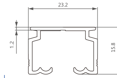
型号/Item No.-13031323 米重/Weight-0.226kg/m
