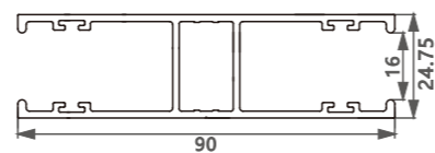
型号/Item No.-79081139 米重/Weight-1.133kg/m
