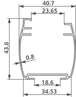
型号/Item No.-13031110-0.8 米重/Weight-0.378kg/m
