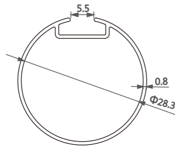
型号/Item No.-11181076-0.8 米重/Weight-0.224kg/m
