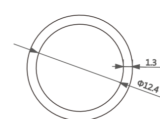
型号/Item No.-611095 米重/Weight-0.153kg/m
