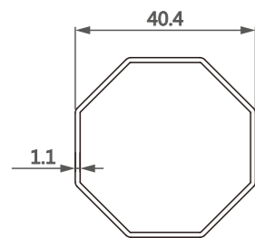
型号/Item No.-191012 米重/Weight-0.387kg/m
