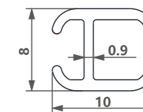
型号/Item No.-1514874 米重/Weight-0.076kg/m
