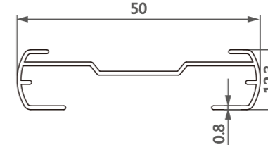
型号/Item No.-1514682 米重/Weight-0.245kg/m
