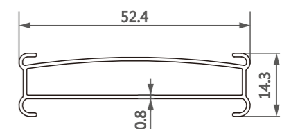
型号/Item No.-13031330 米重/Weight-0.301kg/m
