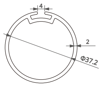
型号/Item No.-1118900 米重/Weight-0.734kg/m
