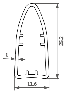
型号/Item No.-1116077 米重/Weight-0.183kg/m
