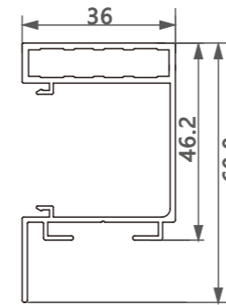
型号/Item No.-19071463 米重/Weight-0.699kg/m
