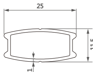
型号/Item No.-11161185 米重/Weight-0.182kg/m
