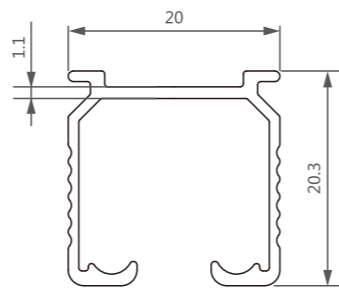
型号/Item No.-1303844 米重/Weight-0.204kg/m
