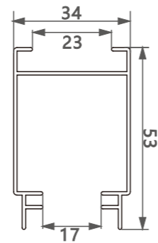
型号/Item No.-13031243 米重/Weight-0.465kg/m
