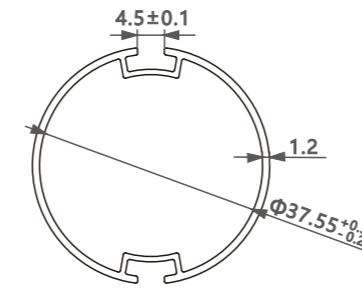
型号/Item No.-1118186 米重/Weight-0.441kg/m
