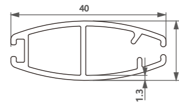
型号/Item No.-1116649-1.3 米重/Weight-0.401kg/m
