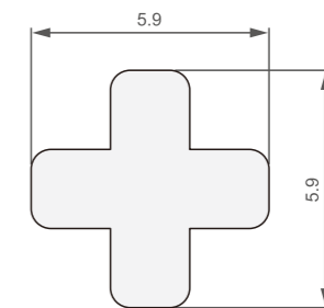
型号/Item No.-130312 米重/Weight-0.053kg/m
