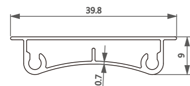
型号/Item No.-1116475 米重/Weight-0.218kg/m
