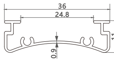
型号/Item No.-110165 米重/Weight-0.189kg/m
