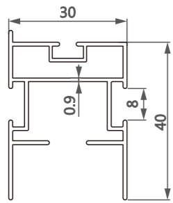
型号/Item No.-13031050 米重/Weight-0.484kg/m
