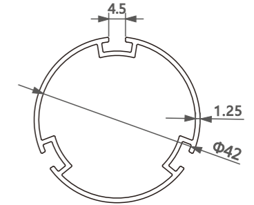
型号/Item No.-1118206 米重/Weight-0.564kg/m
