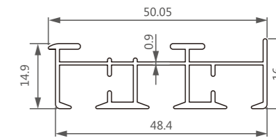
型号/Item No.-1514178 米重/Weight-0.388kg/m
