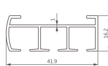
型号/Item No.-151471 米重/Weight-0.355kg/m
