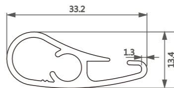
型号/Item No.-1118695 米重/Weight-0.298kg/m
