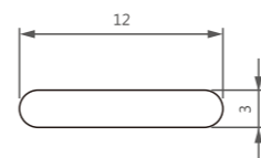
型号/Item No.-920011 米重/Weight-0.093kg/m
