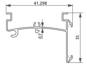
型号/Item No.-111368 米重/Weight-0.242kg/m
