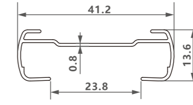
型号/Item No.-1514714 米重/Weight-0.193kg/m
