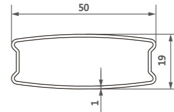
型号/Item No.-11161547 米重/Weight-0.348kg/m
