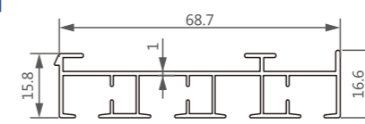
型号/Item No.-1514832 米重/Weight-0.508kg/m
