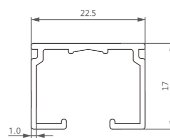
型号/Item No.-13031425 米重/Weight-0.215kg/m
