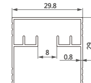
型号/Item No.-79081085 米重/Weight-0.259kg/m
