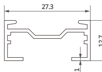
型号/Item No.-1514112 米重/Weight-0.198kg/m
