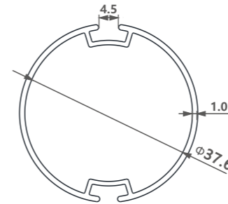
型号/Item No.-1118974 米重/Weight-0.447kg/m
