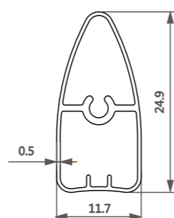
型号/Item No.-11161429 米重/Weight-0.126kg/m
