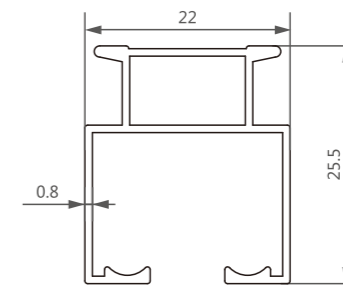
型号/Item No.-1303898 米重/Weight-0.244kg/m
