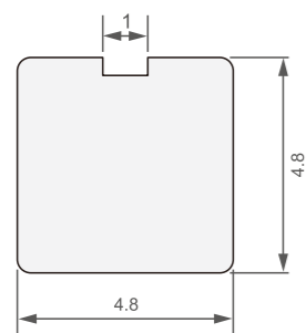
型号/Item No.-1303209 米重/Weight-0.062kg/m
