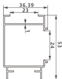
型号/Item No.-13031244 米重/Weight-0.461kg/m
