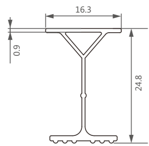
型号/Item No.-1404137 米重/Weight-0.152kg/m
