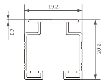
型号/Item No.-13031308 米重/Weight-0.162kg/m
