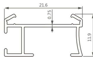
型号/Item No.-110173 米重/Weight-0.121kg/m
