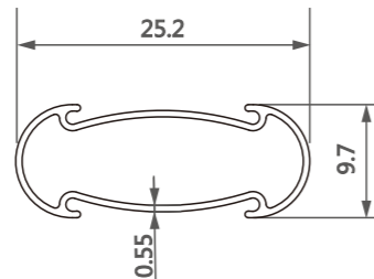
型号/Item No.-11161550 米重/Weight-0.106kg/m
