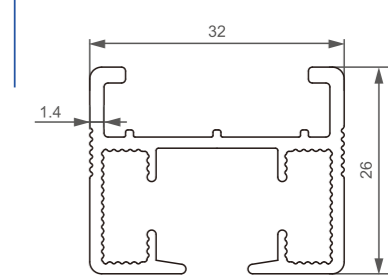
型号/Item No.-1303901 米重/Weight-0.51kg/m
