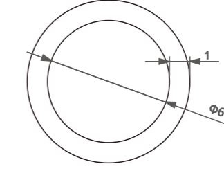
型号/Item No.-6110172 米重/Weight-0.060kg/m
