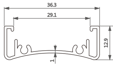
型号/Item No.-110181 米重/Weight-0.256kg/m
