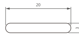
型号/Item No.-920046 米重/Weight-0.159kg/m
