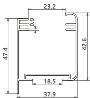
型号/Item No.-1202680 米重/Weight-0.452kg/m
