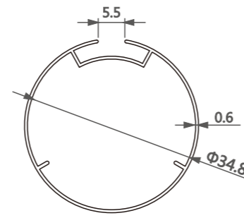
型号/Item No.-1110166 米重/Weight-0.215kg/m
