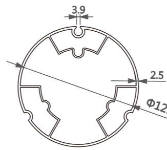
型号/Item No.-11181170 米重/Weight-4.205kg/m
