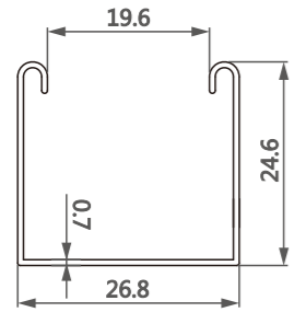
型号/Item No.-1202285 米重/Weight-0.160kg/m
