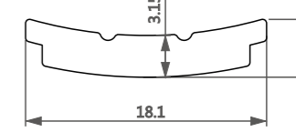
型号/Item No.-11161363 米重/Weight-0.144kg/m
