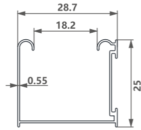
型号/Item No.-11161551 米重/Weight-0.149kg/m
