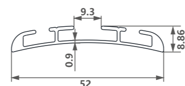
型号/Item No.-11162016 米重/Weight-0.317kg/m
