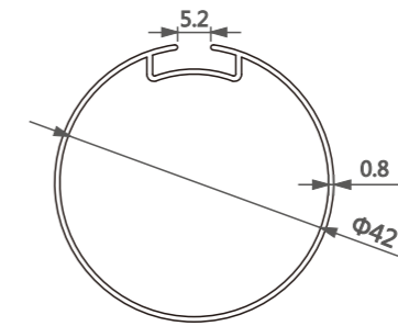
型号/Item No.-1110104 米重/Weight-0.326kg/m
