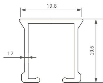
型号/Item No.-1514154 米重/Weight-0.235kg/m
