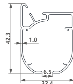
型号/Item No.-11181619 米重/Weight-0.427kg/m
