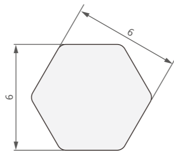
型号/Item No.-191137 米重/Weight-0.085kg/m
