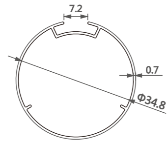
型号/Item No.-1110179 米重/Weight-0.239kg/m
