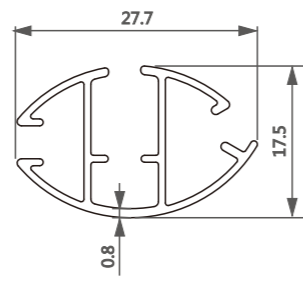
型号/Item No.-11181356 米重/Weight-0.224kg/m
