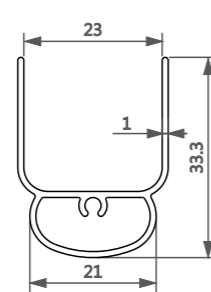
型号/Item No.-1118942 米重/Weight-0.290kg/m
