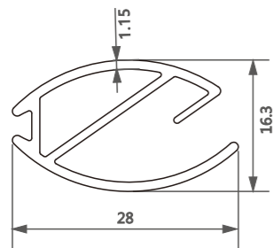
型号/Item No.-1118147 米重/Weight-0.267kg/m
