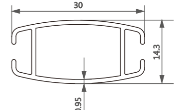
型号/Item No.-11161181 米重/Weight-0.234kg/m
