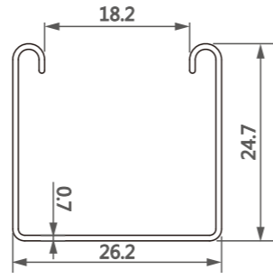
型号/Item No.-120268 米重/Weight-0.158kg/m
