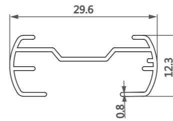
型号/Item No.-1514681 米重/Weight-0.165kg/m
