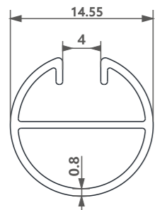
型号/Item No.-11162217 米重/Weight-0.122kg/m
