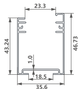
型号/Item No.-1202719 米重/Weight-0.426kg/m
