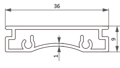
型号/Item No.-111301 米重/Weight-0.318kg/m
