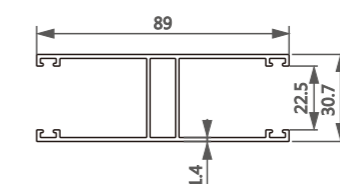
型号/Item No.-4278329 米重/Weight-0.961kg/m
