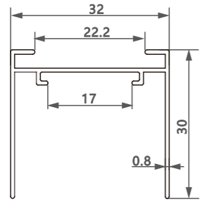
型号/Item No.-13031581 米重/Weight-0.234kg/m
