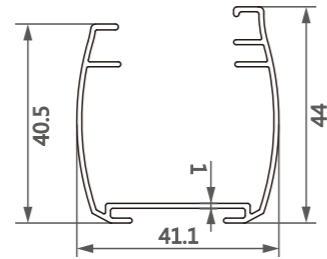
型号/Item No.-13031110 米重/Weight-0.438kg/m
