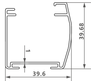
型号/Item No.-1202486 米重/Weight-0.416kg/m
